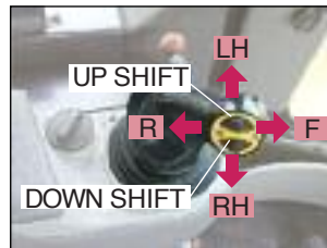
Left-hand Joystick
