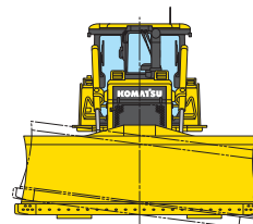
Shown with Power Angle Tilt dozer (D65EX-17) single grouser shoe.
