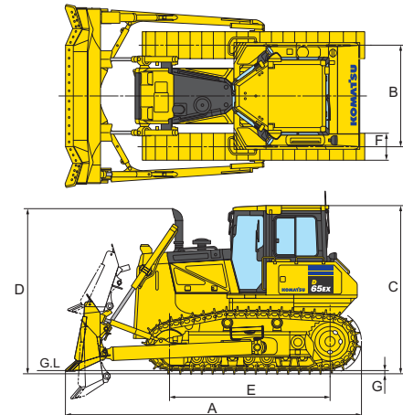
Shown with SIGMADOZER (D65EX-17) single grouser shoe.
