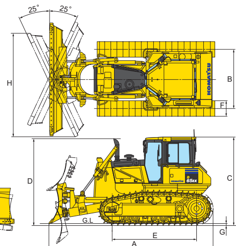
Shown with Power Angle Tilt dozer (D65EX-17) single grouser shoe.
